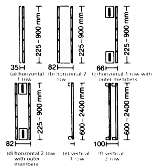
7 Summary of different panel radiators
